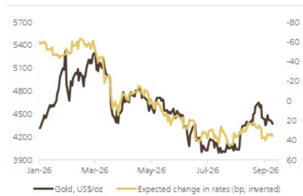
Figure 1: US rates continue to matter, although maybe less so than in previous cycles
