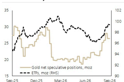
Figure 2: Net speculative long futures positions were washed out as Fed rate hikes repriced, but ETF holdings have been relatively resilient
